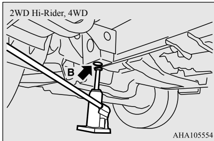
B- Front jacking point (vehicles for 2WD Hi-Rider or 4WD)
