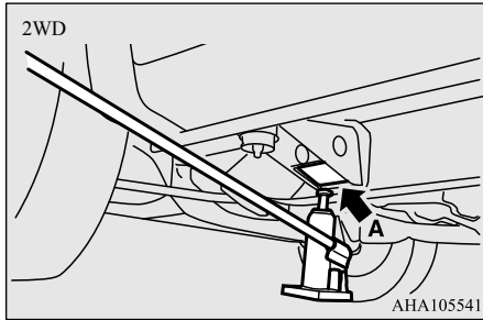
A- Front jacking point (vehicles for 2WD)
