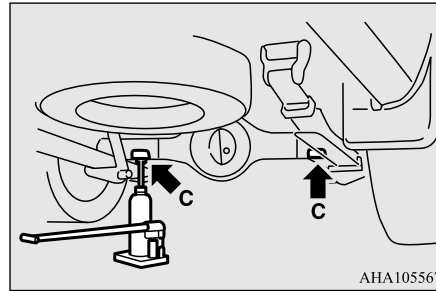
C- Rear jacking point
