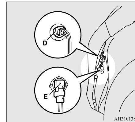
D- Daytime running lamp E- Front fog lamp
