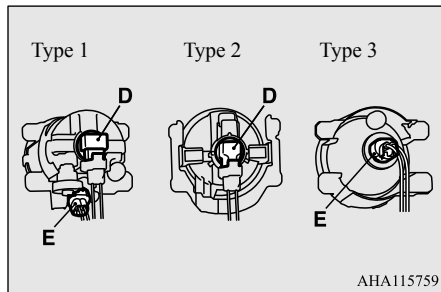
D- Front fog lamp E- Daytime running lamp
